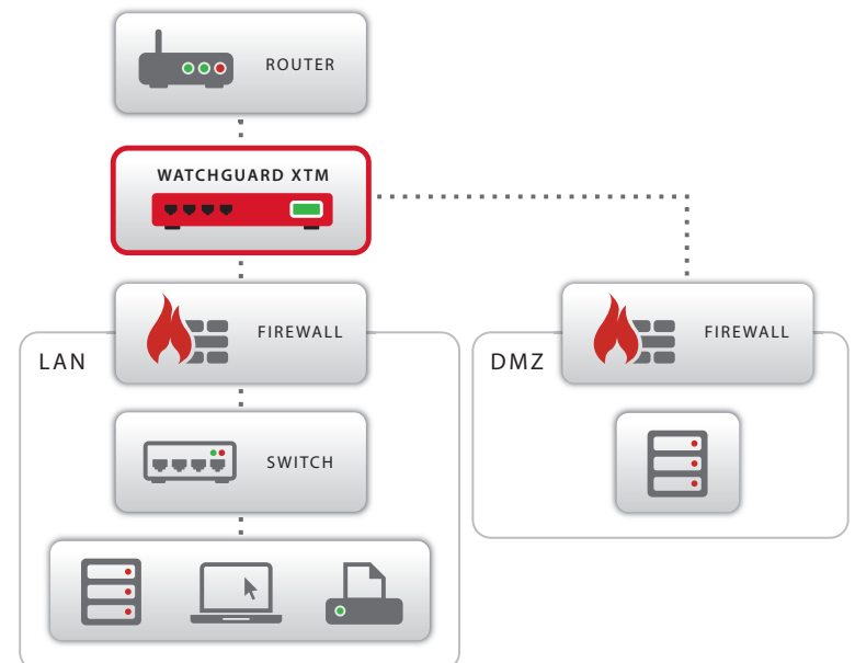
Complex Network with WatchGuard XTM installed in bridge mode between the existing router and firewall
