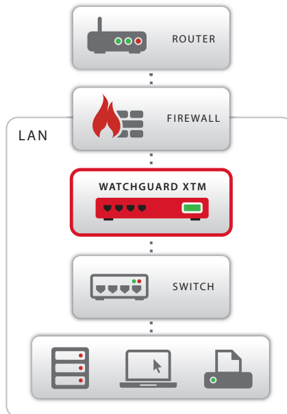
Simple Network with WatchGuard XTM installed in bridge mode between the existing firewall and switch
